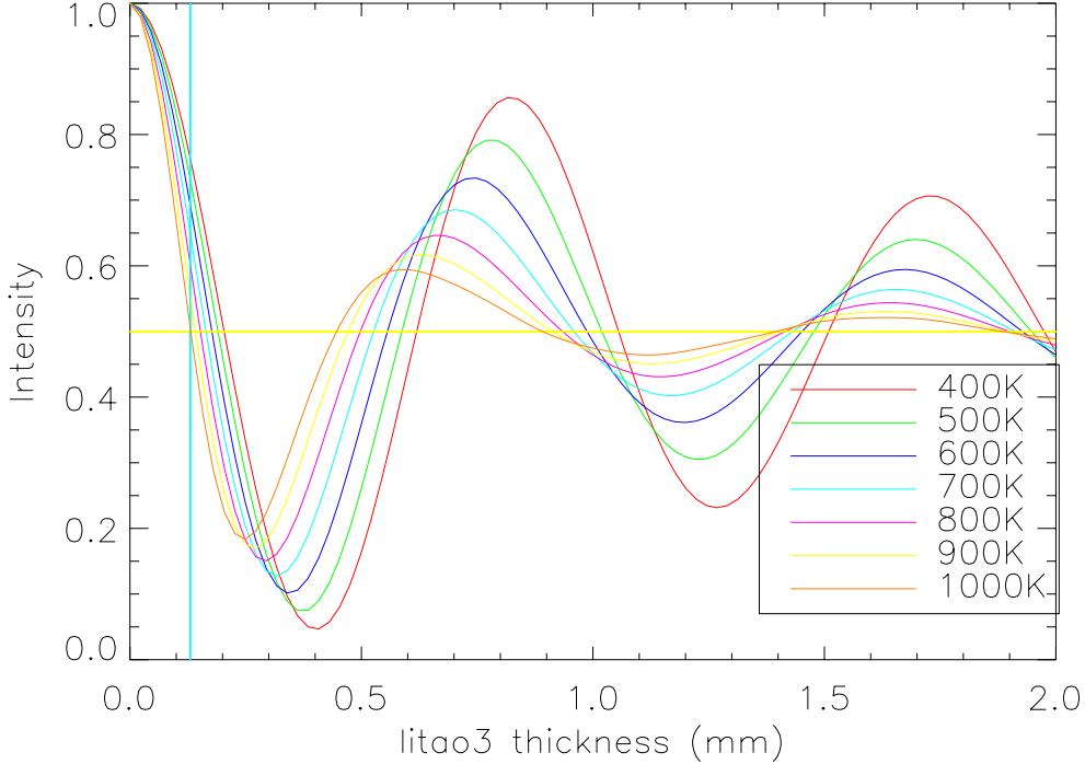
Figure 7: Fourier transform of the emission spectra of Fig. 1. A top-hat bandpass filter spanning the range 1\text{-}5\ \mu\text{m} has been applied. The delay coordinate is expressed in terms of an equivalent thickness of \text{LiTaO}_3 as discussed in the text.
