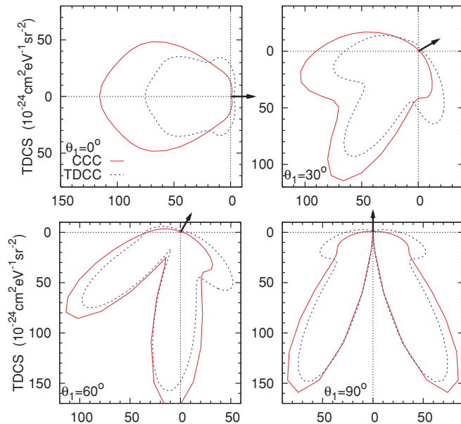
FIG. 1. (Color online) TDCS of DPI of Li at E_1 = E_2 = 5 eV and various fixed escape angles \theta_1 = 0^\circ, 30^\circ, 60^\circ , and 90^\circ (indicated by the arrow). The CCC calculation is shown by the red solid line whereas the TDCC calculation is displayed with the blue dotted line.
