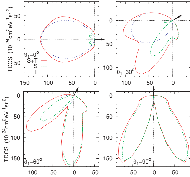
FIG. 3. (Color online) TDCS of DPI of Li at E_1 = E_2 = 5 eV and various fixed escape angles \theta_1 = 0^\circ, 30^\circ, 60^\circ , and 90^\circ (indicated by the arrow). The CCC calculation is plotted with the sum of the singlet and triplet channels (S+T, red solid line), the singlet channel only (S, green dashed line), and triplet channel only (T, blue dotted line).
