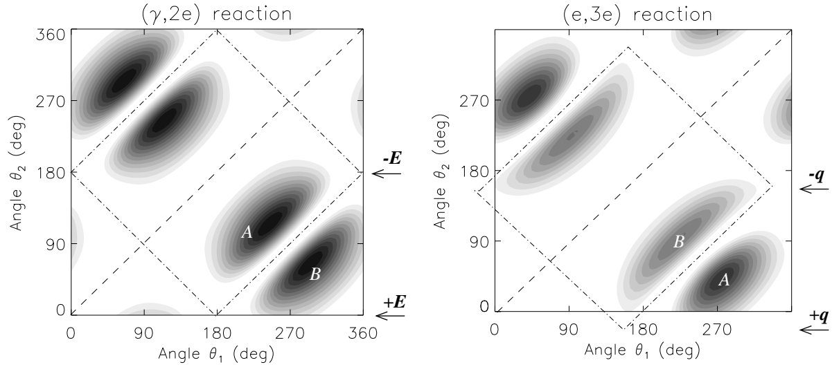
Figure 1. The FBA-CCC calculations of the He (\gamma, 2e) and (e, 3e) fully differential cross sections at ejected electron energies of E_1 = E_2 = 10 eV (left and right panels, respectively). Cross-sections are exhibited in contour plots as functions of the escape angles \theta_1 and \theta_2 . The areas of large cross-section are indicated by darker shades of grey. The straight lines indicate the areas of vanishing cross-section according to the dipole selection rules (dash-dotted lines) and Pauli exclusion principle (dashed line). The arrows show the directions of the electric field vector \pm \mathbf{E} and the momentum transfer vector \pm \mathbf{q} for the (\gamma, 2e) and (e, 3e) reactions, respectively. The angular range accessible in the Orsay experiment contains the peaks denoted by A and B in the plots, see text.
