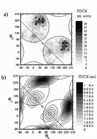
FIG. 2: As for Figure 1 except q = 2 \pm 0.2 a.u.. a) experimental FDCS. b) First Born CCC calculation.
