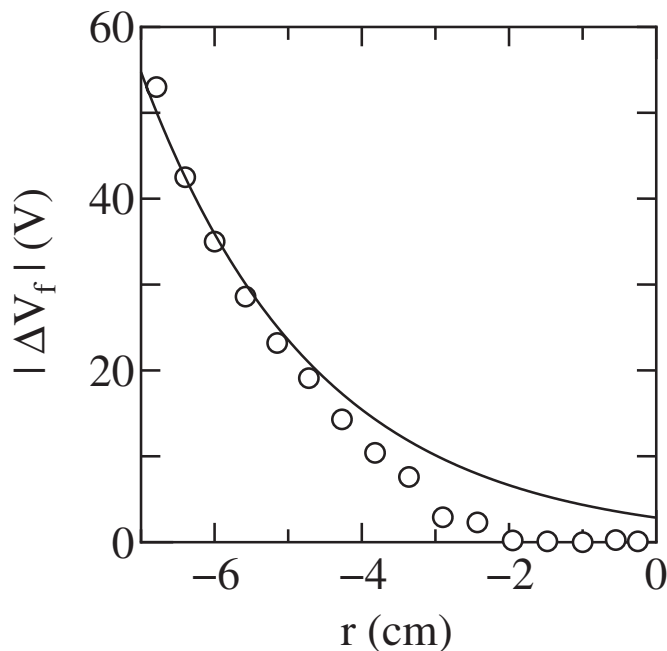
FIG. 5. Open circles are the difference |\Delta V_f| between the left and right measured V_f of Fig. 4, and the solid line is an exponential fit having an e-folding of 2.4 cm.
