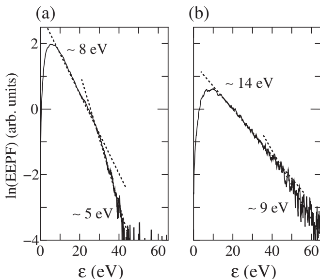
FIG. 2. EEPFs measured using the rf compensated Langmuir probe, respectively, positioned at (a) (z,r)=(17 \text{ cm}, 0 \text{ cm}) (circle 1 in Fig. 1) and at (b) (z,r)=(17 \text{ cm}, 4 \text{ cm}) (circle 2 in Fig. 1); operating conditions are 250 W rf power and 0.3 mTorr gas pressure.
