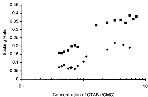
Figure 8. Sticking ratio (determined from the initial rate of adsorption) versus concentration for solutions of CTAB, normalized by the corresponding CMC, with (squares) and without (diamonds) added 10 mM KBr. The values of the variables used in the calculation of the theoretical diffusion-limited flux were as follows: u = 0.0022 , R = 0.0013 , \nu = 8.93 \times 10^{-7} , Re = 3.37 , a = 2 \times 10^{-9} , D(\text{monomer}) = 1.21 \times 10^{-10} , D(\text{micelle}) = 8.36 \times 10^{-11} \text{ m}^2 \text{ s}^{-1} , h = 0.0015 , and \alpha = 6 . The concentration was in kilograms per cubic meter of the surfactant solution. The sticking ratio increases at the CMC for both systems.
