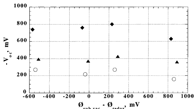
Figure 2. The open circuit photovoltage at 75 mW/cm 2 (~1 sun) plotted vs the difference between the work function of the substrate in vacuum, \Phi_{\text{sub,vac}} , and the solution redox potential, \Phi_{\text{redox}} . The work function of the substrate in the solution, \Phi_{\text{sub}} , the quantity of interest, is difficult to measure but is related to \Phi_{\text{sub,vac}} , see the discussion in the text. The four types of substrates are, from left to right, ITO, SnO 2 , Au, and Pt; the filled diamonds are for 0.5 M LiI solution, the open circles are for 0.05 M ferrocene in 0.1 M LiClO 4 solution, and the filled triangles are for 0.05 M hydroquinone in 0.1 M LiClO 4 solution.
