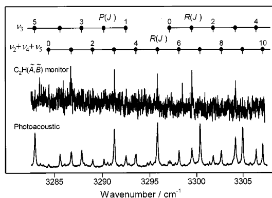
FIG. 4. The IR-VUV double resonance excitation spectrum of C_2H_2 (upper) obtained by scanning the IR-laser wave number while monitoring the fluorescence emitted from the C_2H(\bar{A}, \bar{B}) fragments. The VUV laser wave number is tuned to 74 522 cm^{-1} , where the \bar{F}-\bar{X} 3_1^1 band is located. The photoacoustic (PA) excitation spectrum in the IR range (lower) observed simultaneously is compared. As shown in the rotational assignments, the two vibrational bands, i.e., \nu_3'' and \nu_2'' + \nu_4'' + \nu_5'' , overlap with each other in this IR range.
